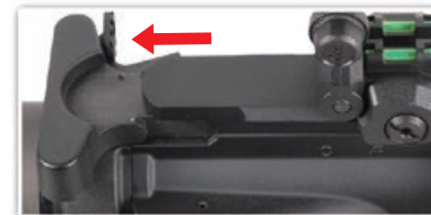
Pulling the charging handle will take the bolt back and open the port cover.
